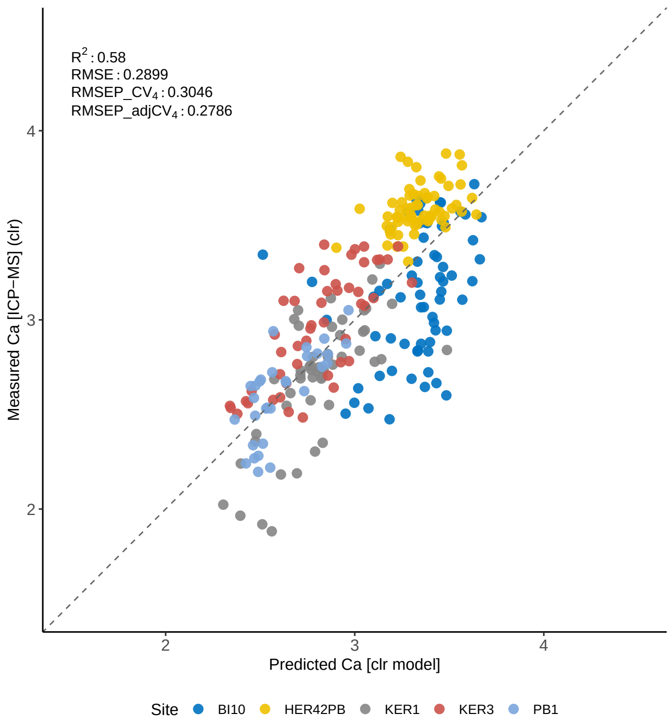
PLSR: Measured vs Predicted Ca: clr model
